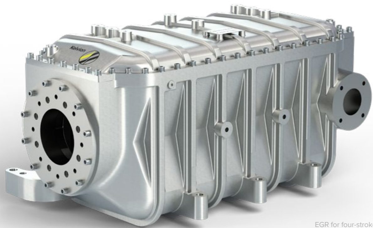
EGR for four-stroke Engines
