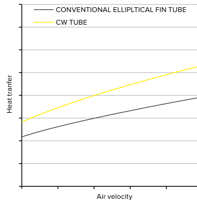
Heat transfer
