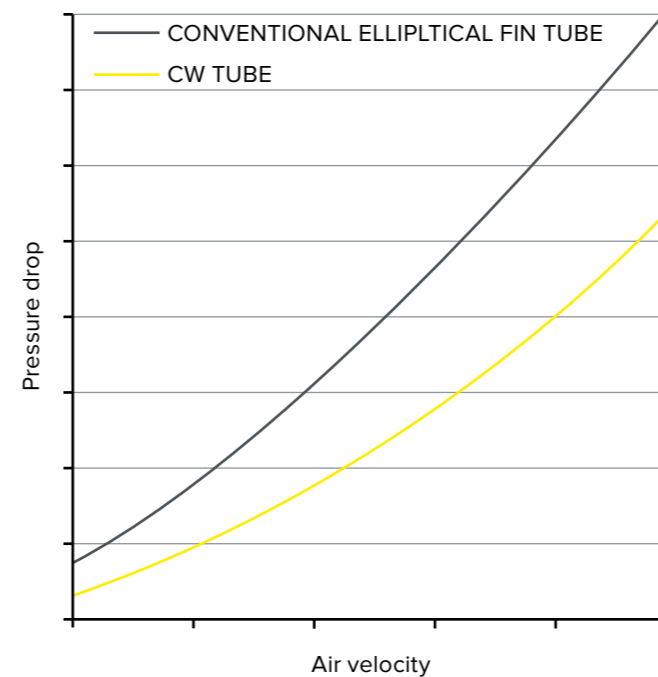
Pressure drop
