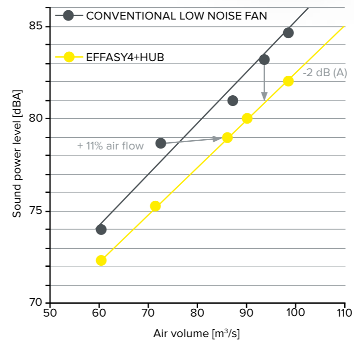
EFFASY fan - Sound power level
